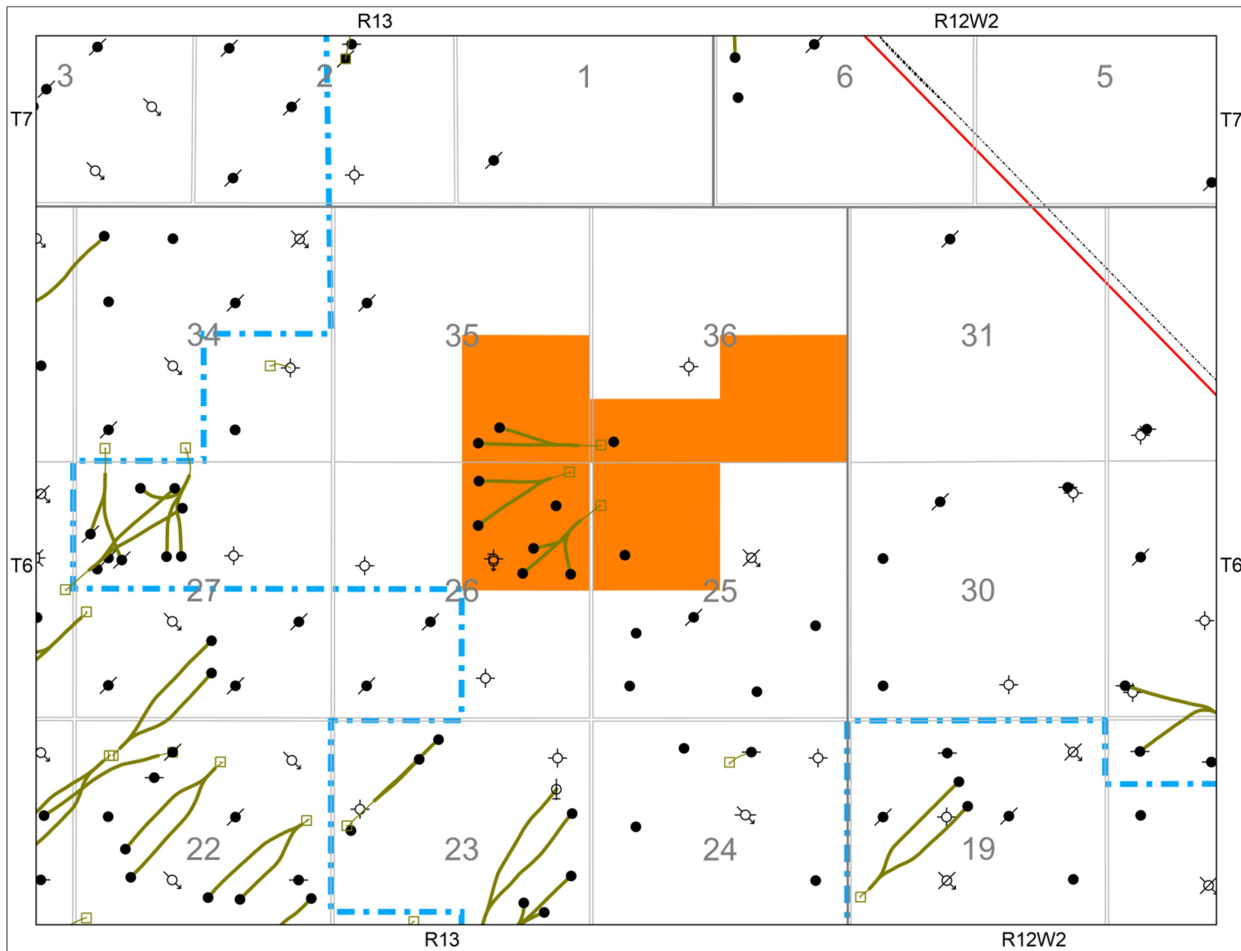
Figure 1: The Weyburn property is highlighted orange and the edge of the Weyburn Unit is delineated by the blue dashed line.
